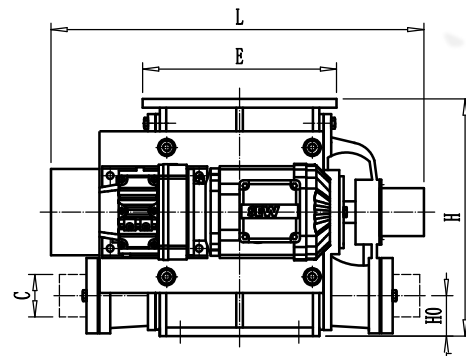
贯通正压关风器 BFCP Blow-through Rotary Airlock Valve
